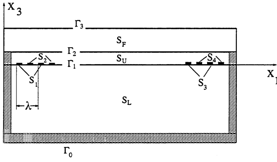
Figure 2: Two-dimensional model
